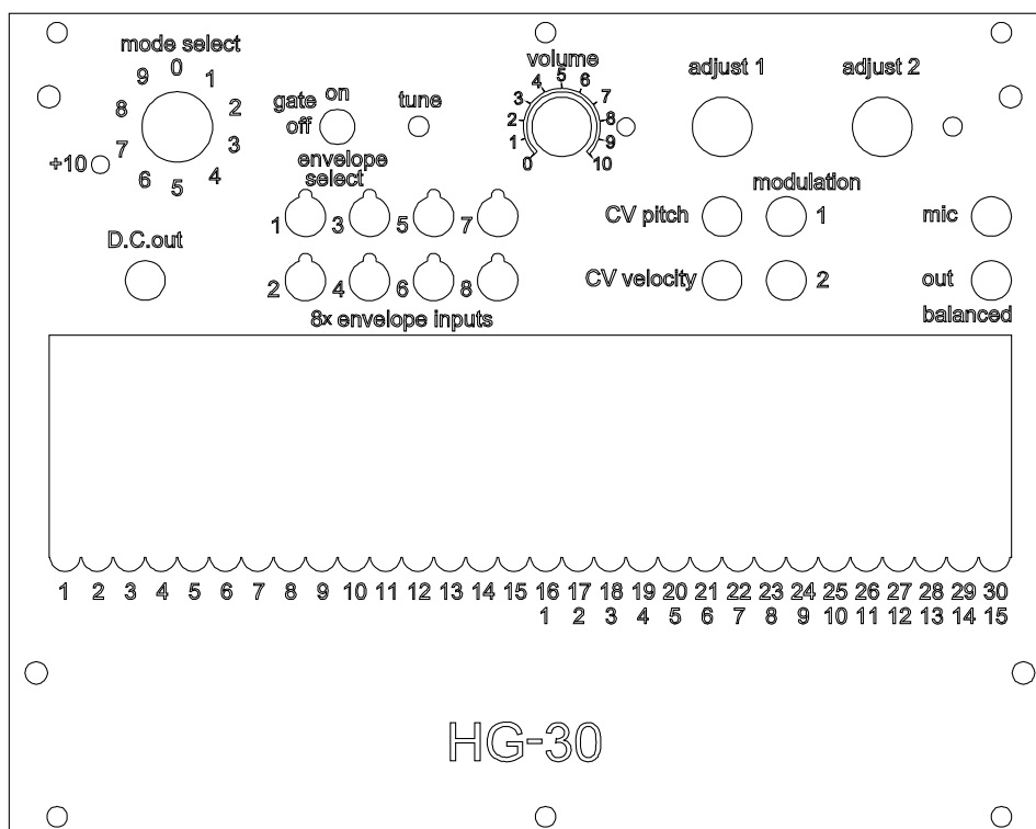
Figure 1: The HG-30 front panel texts and outlines.
